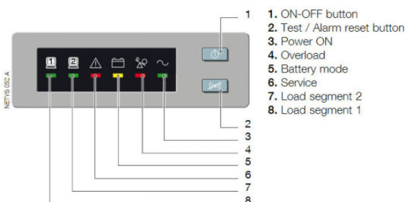
Control panel
